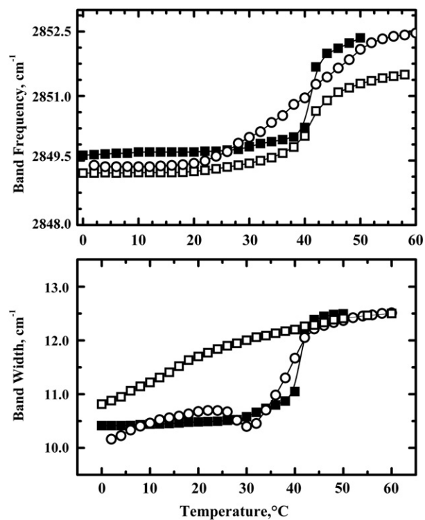
Fig. 10. Temperature-dependent changes of the properties of the \text{CH}_2 symmetric stretching band exhibited by sterol-free DPPC bilayers (—■—), and by DPPC bilayers containing ~30 mol% cholesterol (—□—) and ~30 mol% ergosterol (—○—). The data shown were obtained by analyses of spectra acquired in the heating mode with the top panel illustrating the temperature-induced changes in the band maxima and the bottom panel showing the corresponding changes in overall band width.
