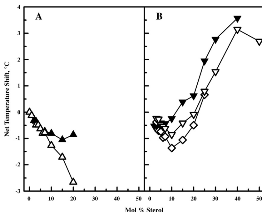
Fig. 8. The net temperature shift of the sharp and broad components of the main chain melting phase transition of cholesterol (▲,▼) and ergosterol/DPPC (△, ▽, ◇) samples obtained from DSC heating thermograms relative to that of pure DPPC. Two broad components exist in the ergosterol samples which are depicted here as either an empty inverted triangle (upper temperature component) or an empty diamond (lower temperature component).
